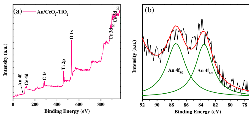
Figure 4. XPS survey spectrum of Au/CeO 2 -TiO 2 nano-hybrid (a), and high resolution XP spectrum of Au 4f (b).
