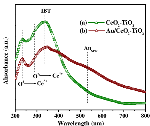
Figure 3. Diffuse reflectance UV-Vis spectrum of (a) CeO 2 -TiO 2 , and (b) Au/CeO 2 -TiO 2 nano-hybrid.
