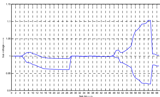
Fig.7 voltage profile for 90% load with &without DGs connected.
