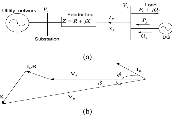
Fig. 1 (a). Utility network with wind DG system (b) phasor diagram
