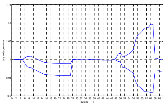
Fig.4 voltage profile for full load with & without DGs connected.
