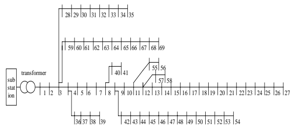
Fig. 3 Radial distribution feeder with 69 buses
