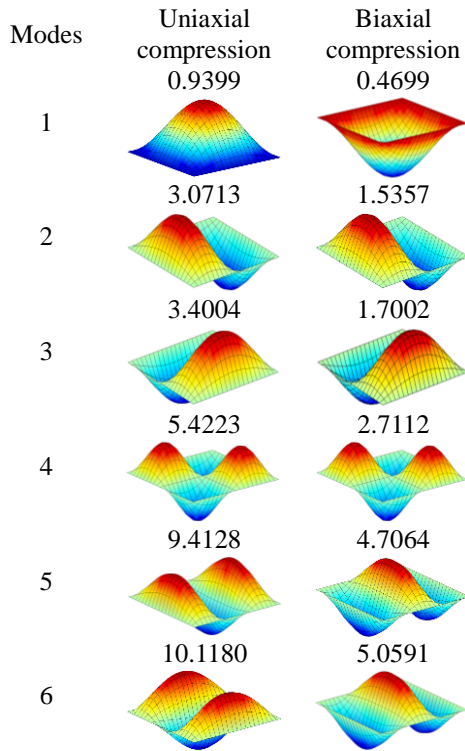
Fig. 3 Comparison of first six buckling mode shapes of B/F/B MEE plate subjected to uniaxial and biaxial compression for CCCC boundary ( a/b=1 , a/h=100 )
